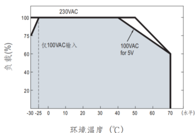
降额曲线:
