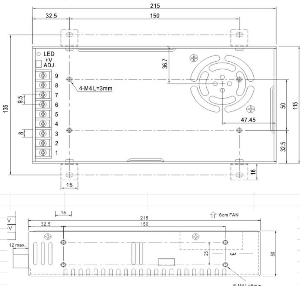
Dimensional drawing of mechanism:
