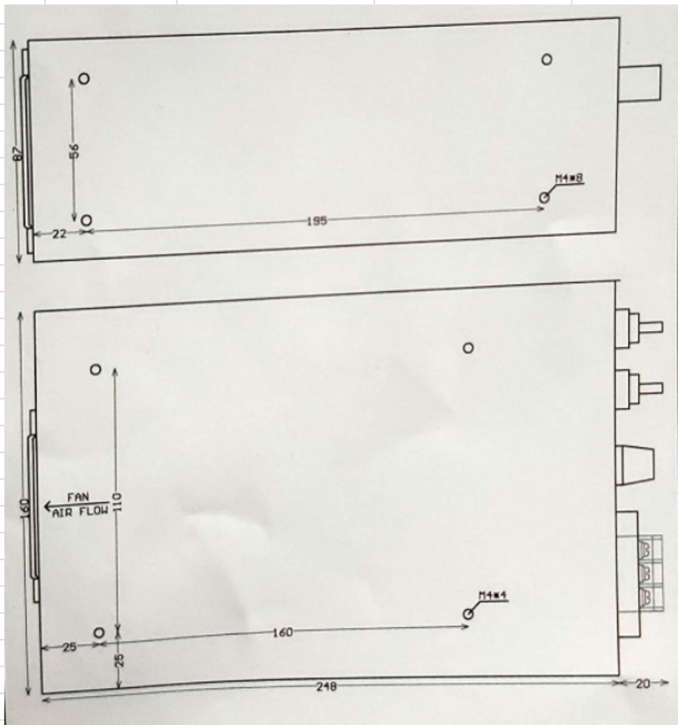
Dimensional drawing of mechanism:
