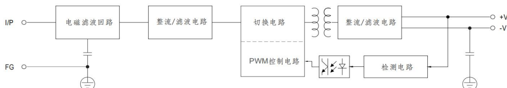
Block diagram of internal mechanism
