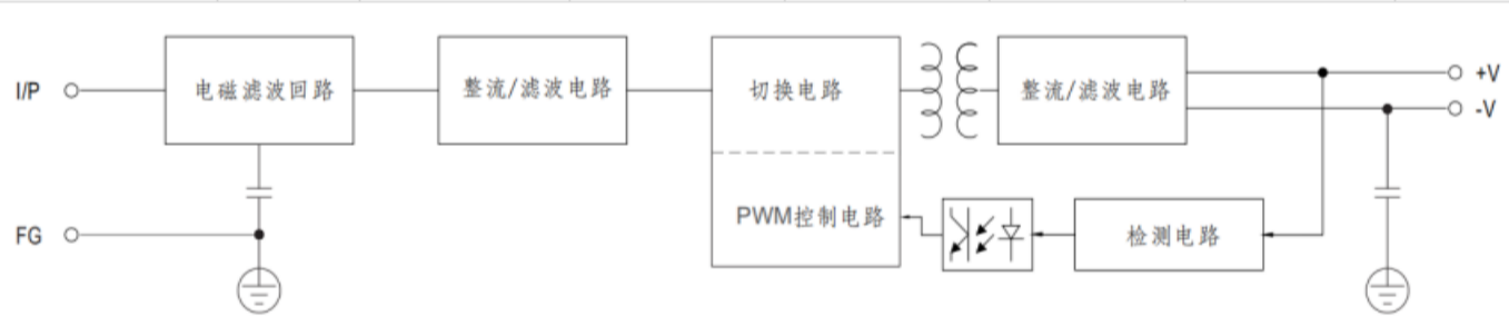
Block diagram of internal mechanism
